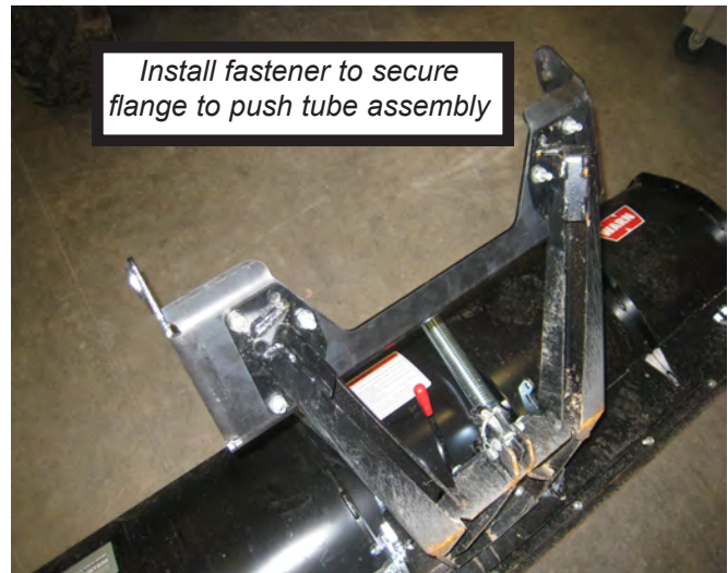
Figure 5 Install fasteners
